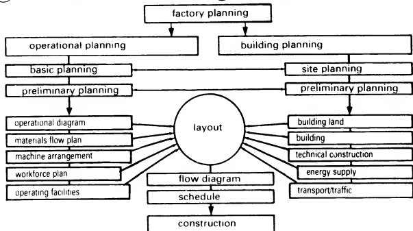
⑧ Planning diagram for a factory
